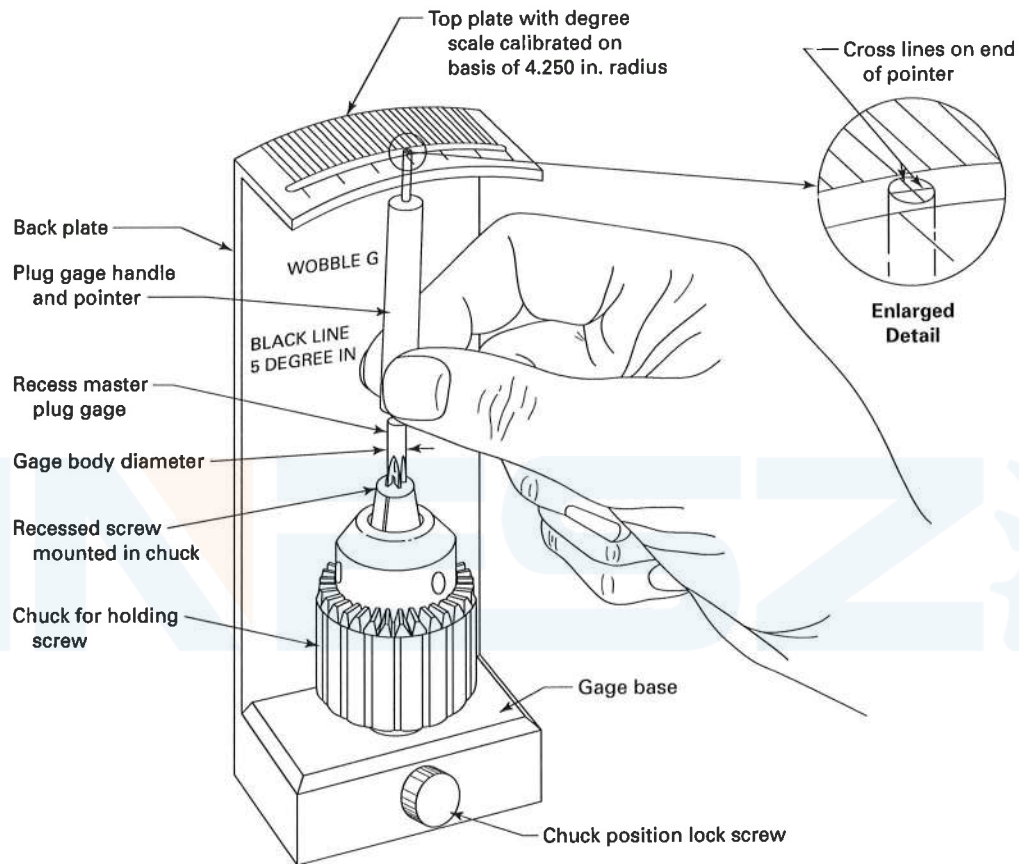
Fig. IV-1 Wobble Gaging Fixture
