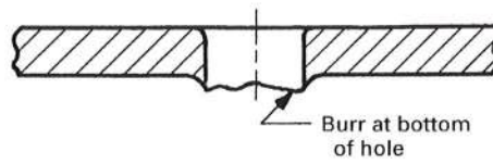
Fig. D-5 Type I Extruded Hole
