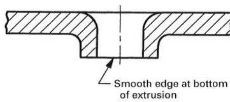
Fig. D-6 Type II Extruded Hole
