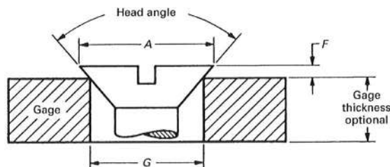
Fig. I-1 Protrusion Gage
