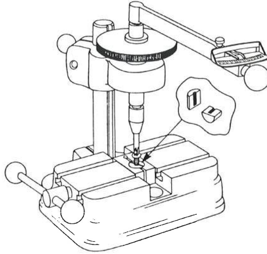
Fig. 4 Typical Torsional Strength Test Fixture
