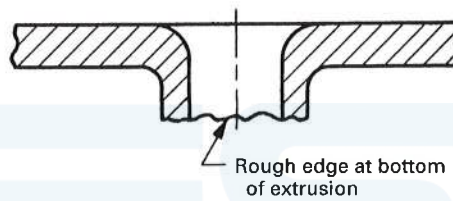
Fig. D-5 Type I Extruded Hole
