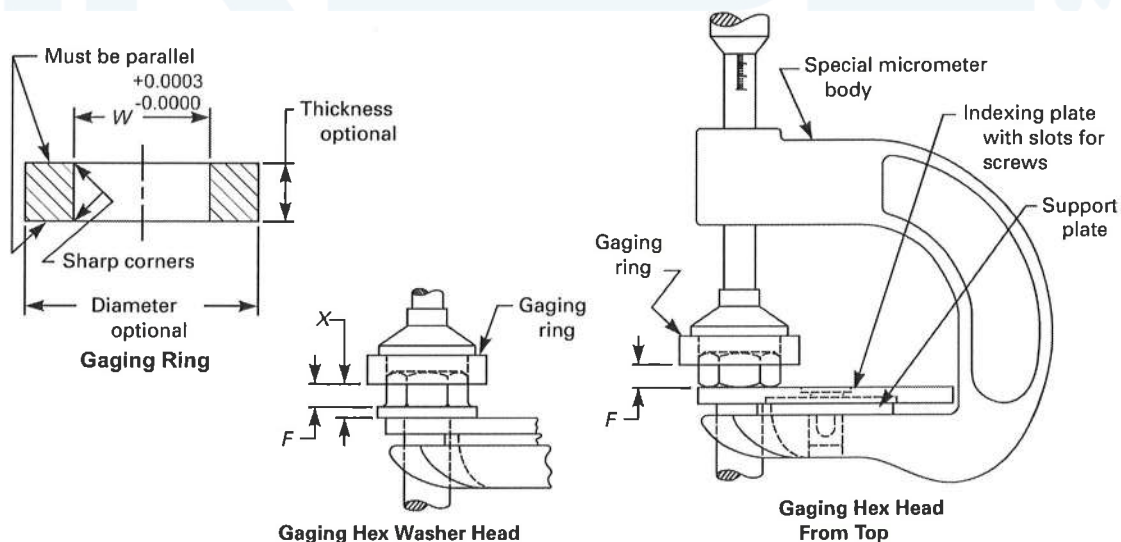
Fig. II-1 Typical Gaging Fixture
